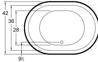
All bathtub dimensions are ± 1/2"
