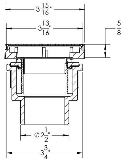
SECTION 1-1
