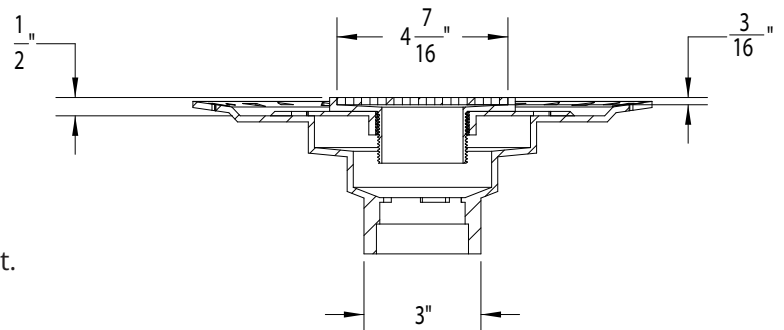
SECTION 1-1
